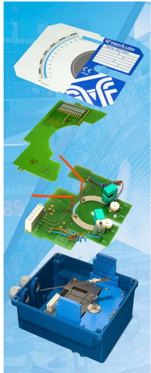
Modular housing
