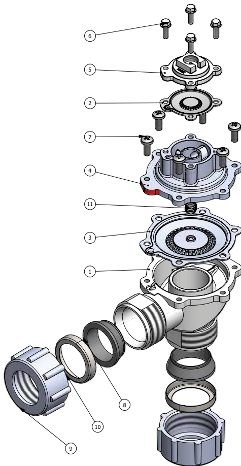
Figure 9: Coupling Connection High Pressure Pulse Valve Without Coil G1 1/2"
