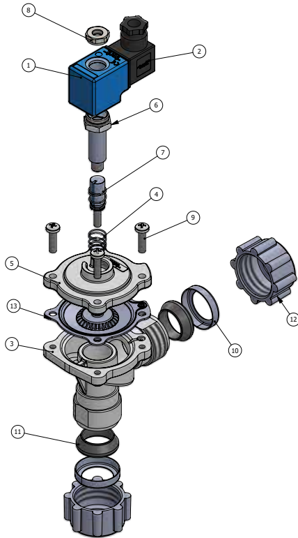
Figure 6: Coupling Connection Standard Pulse Valve With Coil G3/4" - G3/4", G1" - G1"
