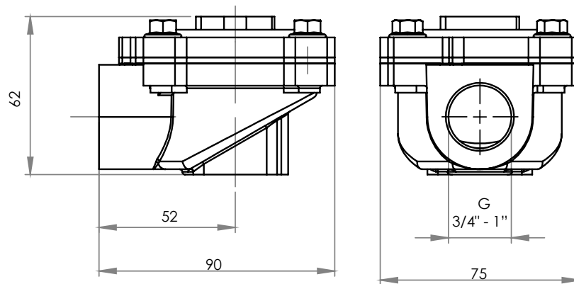
Figure 12: Remote Controlled Pulse Valve Without Coil Sizes G3/4", G1"
