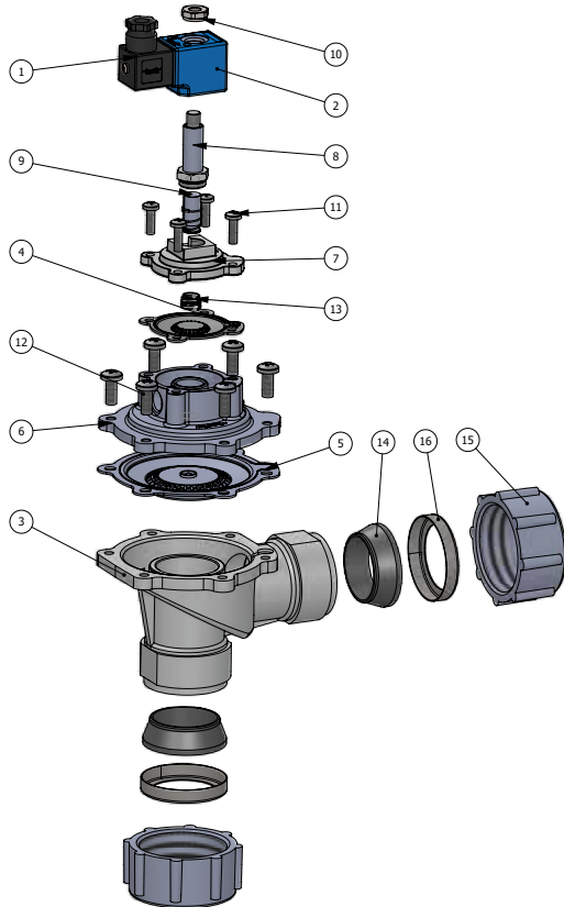
Figure 7: Coupling Connection Standard Pulse Valve With Coil G1 1/2" - G1 1/2"
