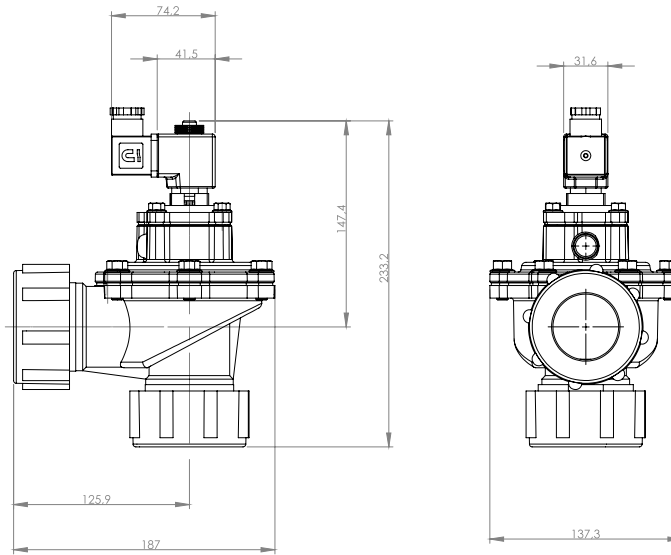
Figure 14: Coupling Connection Standard Pulse Valve With Coil Sizes G3/4", G1", G1 1/2"
