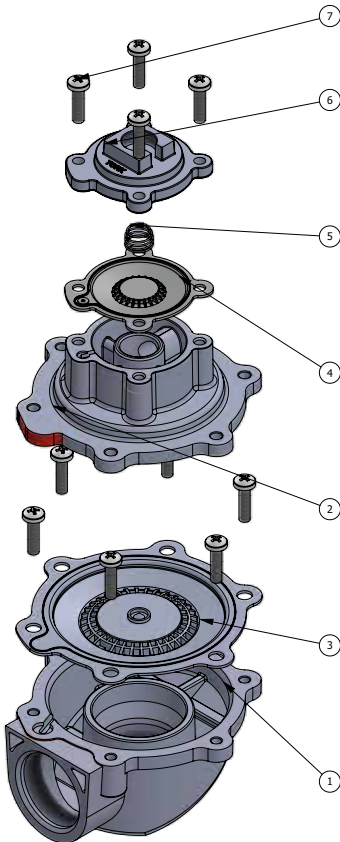
Figure 5: Remote Controlled Pulse Valve Without Coil G1 1/2", G2", G2 1/2", G3"
