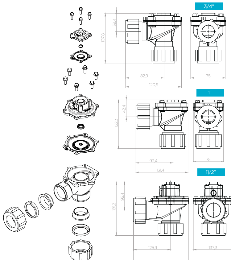
Figure 15: Coupling Connection High Pressure Pulse Valve With Coil Sizes G1 1/2"
