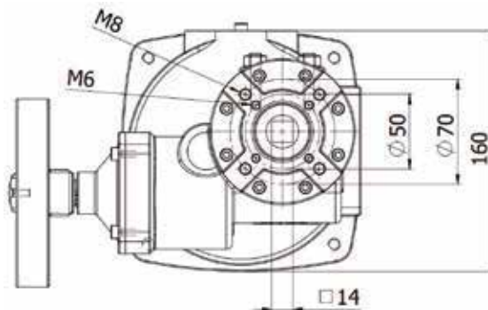
Figure 4. ISO 5211 Sizes
