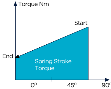
TORK RA ... SR Series (Single Acting) Actuator Output Diagram
