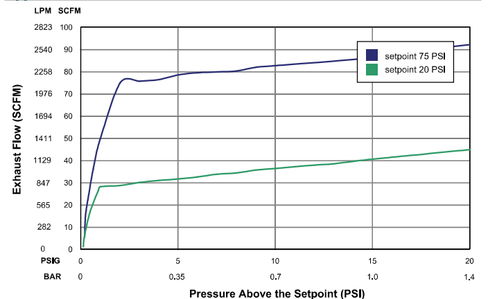
Type 110: Exhaust Curve
