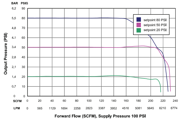
Type 110: Forward Flow Curve, 3/4 and 1 NPT
