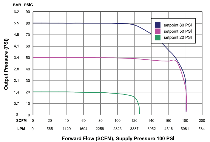
Type 110: Forward Flow Curve, 3/8 and 1/2 NPT
